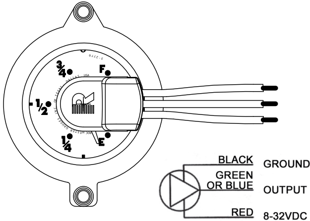
Hall Twinsite® Pin Output Diagram
